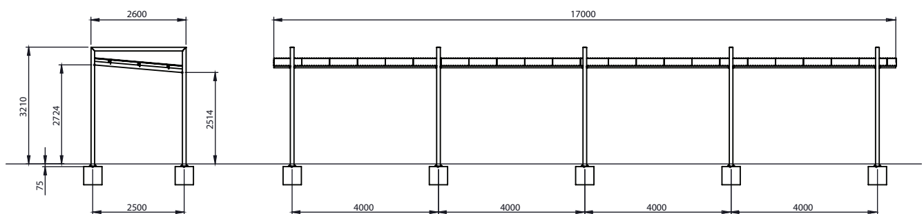
FRONT ELEVATION
