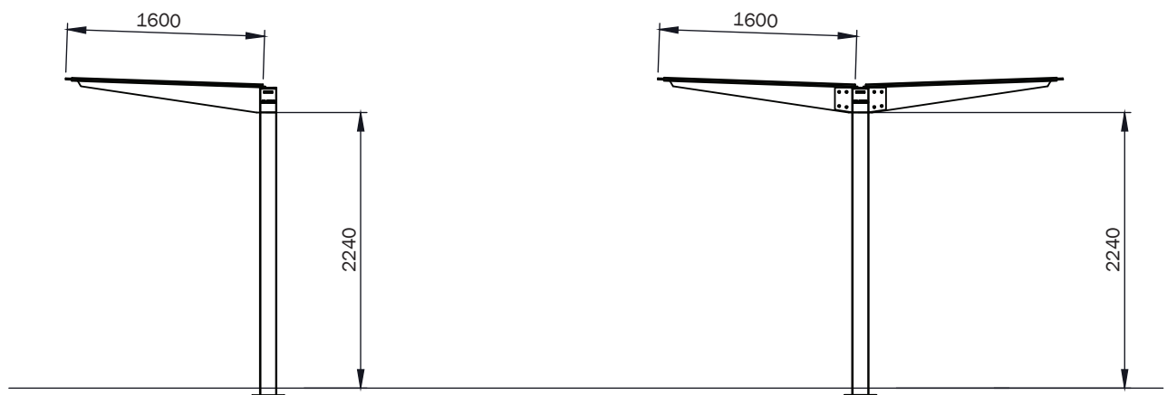
SINGLE SIDED WALKWAY SIDE ELEVATION
